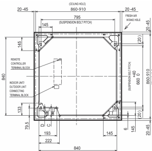
Upper View
